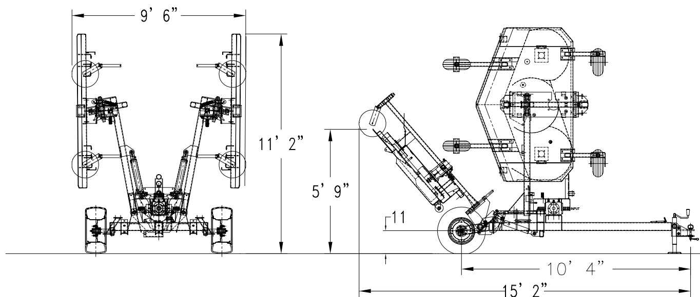
AFM4522 Specification Drawing
