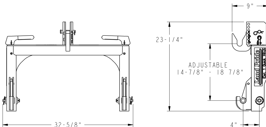
QH15 Quick Hitch Figure 5-1
