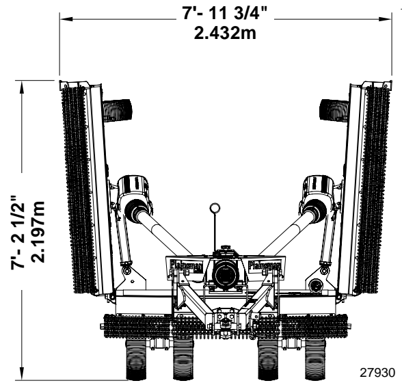
Transport Width With Wing Axles Disconnected At Turnbuckles (#5) And Wheels Folded Back
