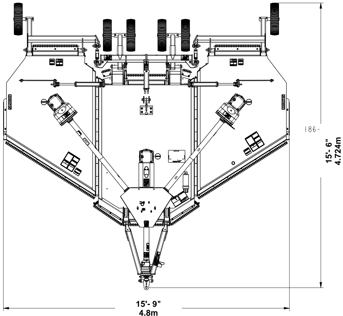
Transport Width Without Special Adjustments
