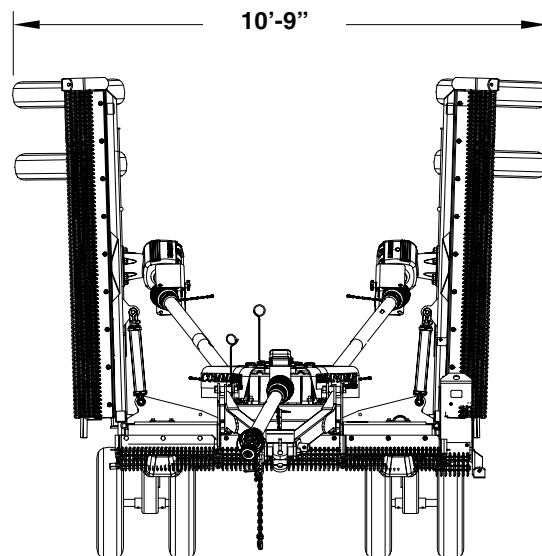
Transport Width Without Special Adjustments
