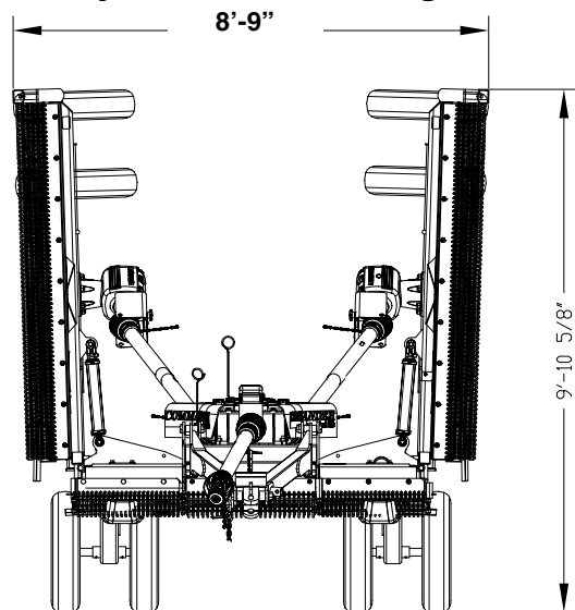
Transport Width With Wing Axes Disconnected At The Turnbuckles And Wheels Folded Back
