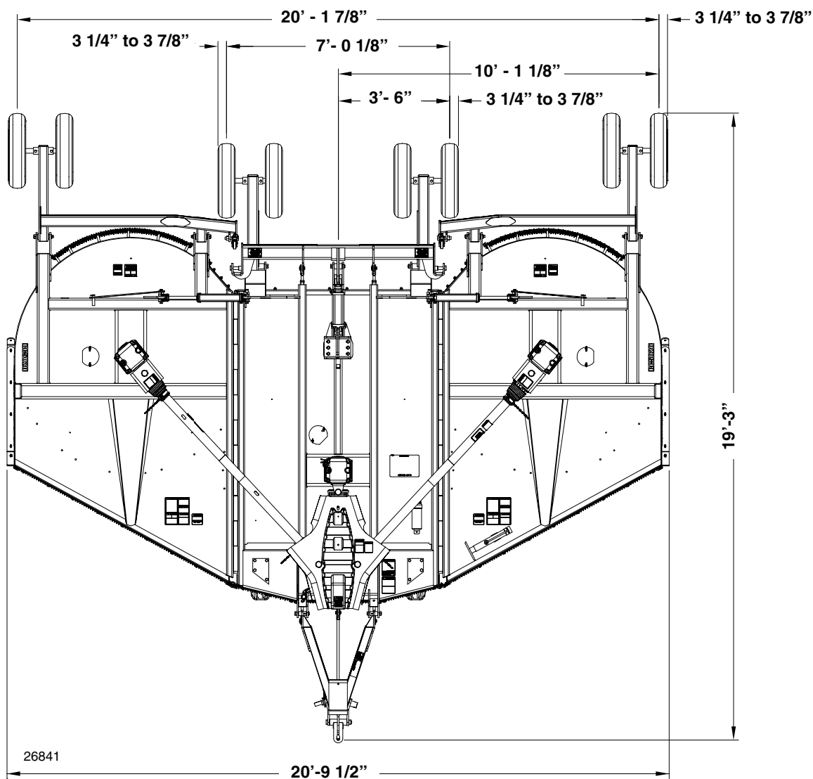
Transport Width Without Special Adjustments
