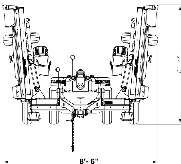
Transport Width Without Special Adjustments. Cylinders Are Fully Retracted
