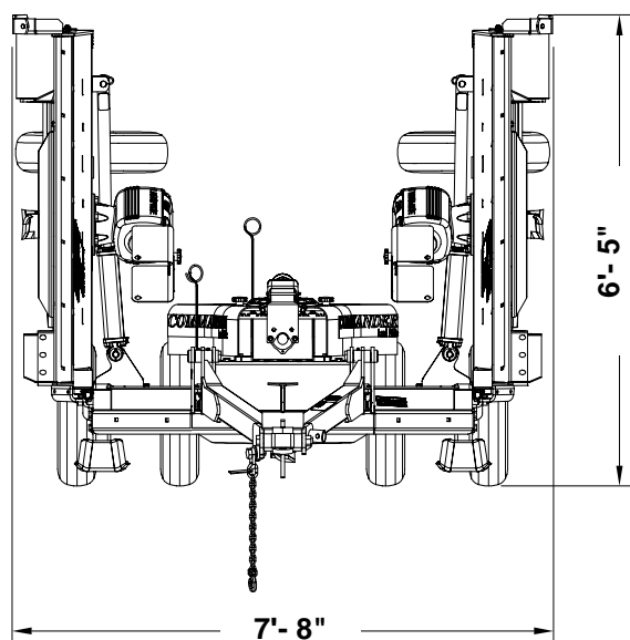
Transport Width With Wing Axles Disconnected At The Turnbuckles And Wheels Folded Back. Cylinders Are Fully Retracted.
