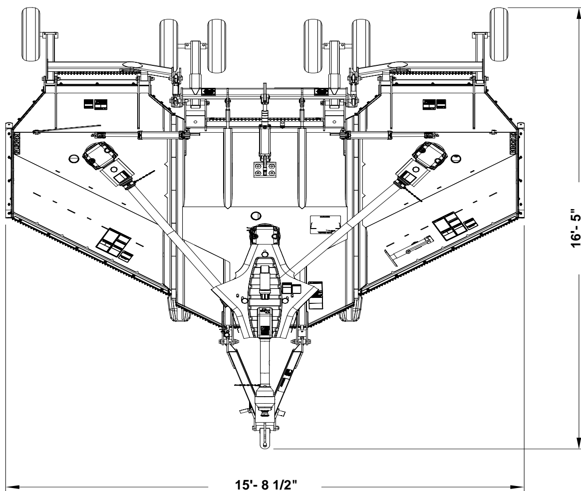
Transport Width With Wing Axles Disconnected At The Turnbuckles And Wheels Folded Back. Cylinders Are Fully Retracted.
