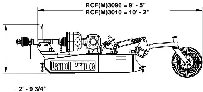
Semi-Mounted Rotary Cutter (RCF3096 Shown)
