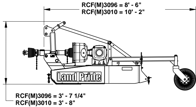
3-Point Mounted Rotary Cutter (RCF3096 Shown)
