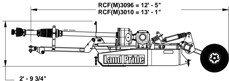
Pull-Type Rotary Cutter (RCF3096 Shown)
